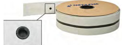
1/2" FEMALE THREADED INTEGRAL WELDED OUTLET * BLACK COLOR - POLYNET GREEN COLOR - FLEXNET
